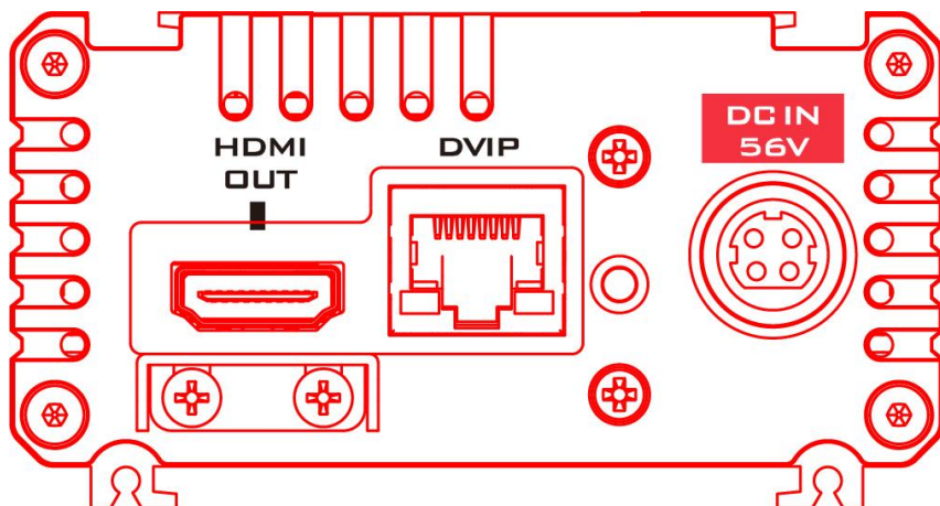
HDMI OUT
